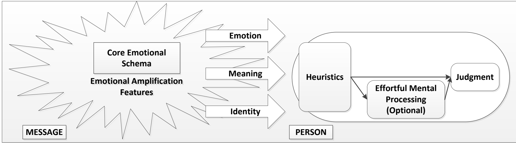
Figure X: Message Processing
